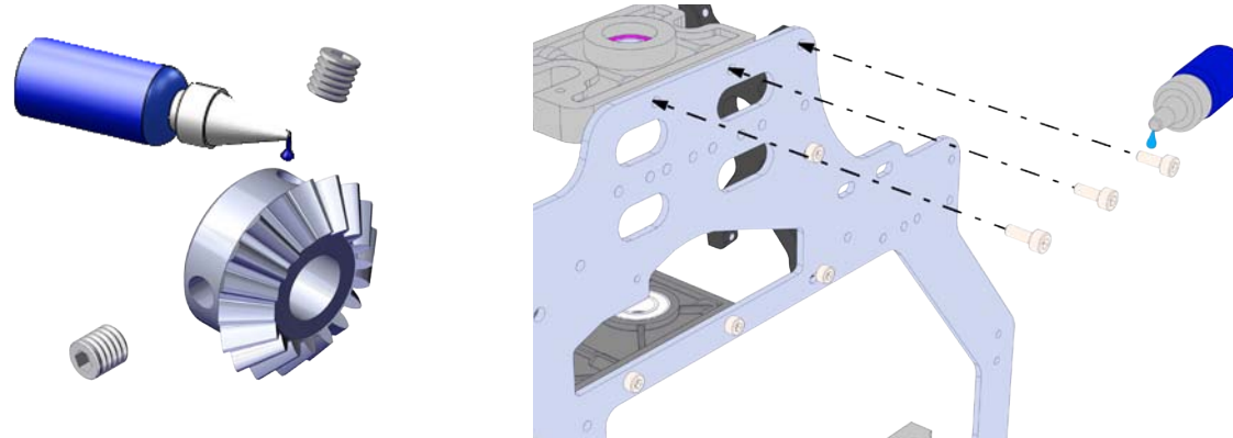
Schraubensicherung, mittelfest, 10 ml Ord.No. 10/24 Thread-lock fluid medium-strength, 10 ml Ord.No. 10/24
